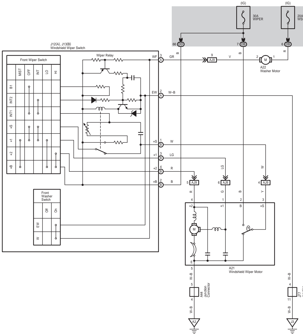
Front Wiper and Washer (w/ Intermittent Wiper)
