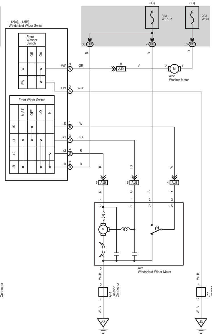
Front Wiper and Washer (w/o Intermittent Wiper)
